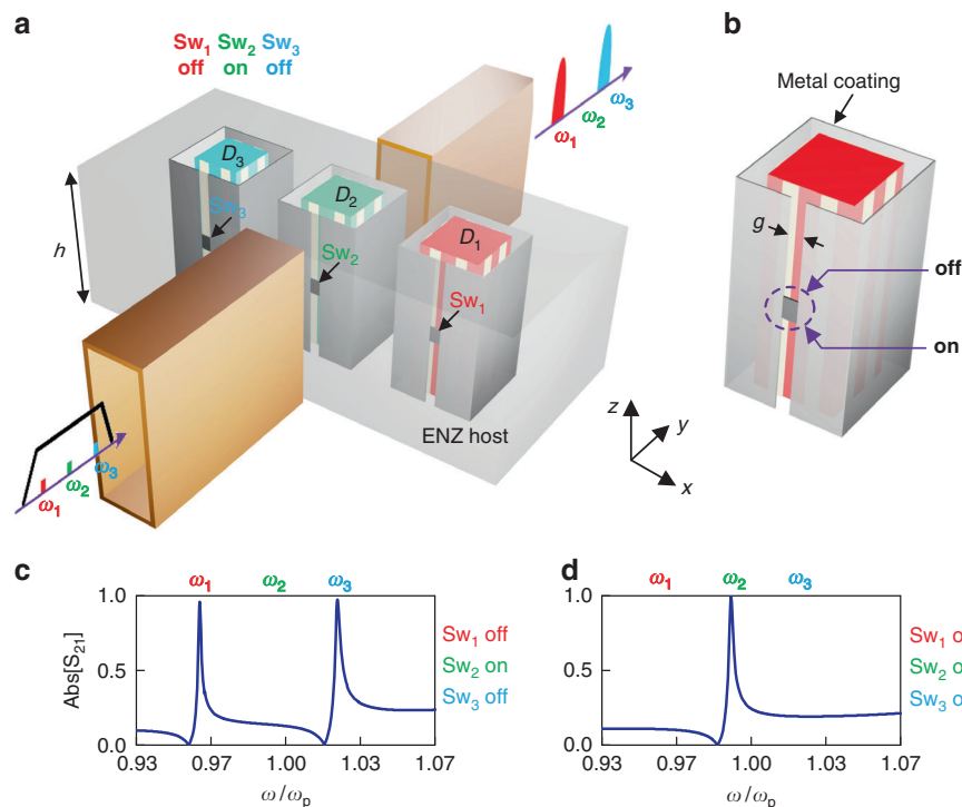
Fig. 5 Multi-frequency dynamic filtering. a The architecture and working principle of the proposed three channel dynamic filter, where multiple dopants controlled by switches independently govern narrow channels at angular frequencies \omega_1 , \omega_2 , and \omega_3 . The metallic cavity is designed with a height h of 0.5\lambda_p ( \lambda_p is the free-space wavelength at \omega_p = 2\pi \times 3 \times 10^9 rad/s). Side lengths of square cross-sections of the dopants D_1 , D_2 , and D_3 are 0.112\lambda_p , 0.106\lambda_p , and 0.097\lambda_p , respectively. The metallic side walls of the doped cavity are not shown here. (b) Configuration of a photonic dopant assembled with a switch. (c) and (d) are the simulation results for the transmitting spectra under different states of the switches
