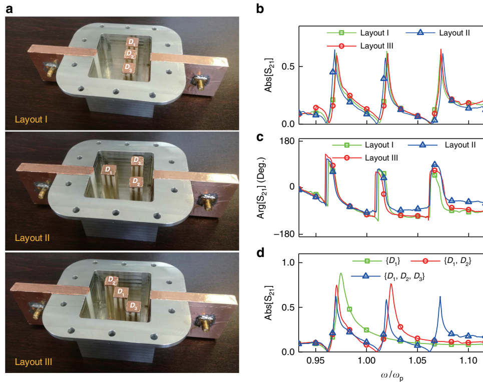
Fig. 4 Experimental verification. a The photograph of the experimental setup. Three cuboid ceramic blocks ( D_1 , D_2 , and D_3 ) with permittivity \varepsilon_1 = 37 and cross-sectional areas of 0.122\lambda_p \times 0.122\lambda_p , 0.116\lambda_p \times 0.116\lambda_p , and 0.11\lambda_p \times 0.11\lambda_p ( \lambda_p is the free-space wavelength at \omega_p = 2\pi \times 3 \times 10^9 rad/s) are arranged in the metallic cavity with a height h of 0.5\lambda_p and a cross-sectional area of 0.66\lambda_p \times 0.5\lambda_p . The upper plate of the metallic cavity is not shown in the photographs. The doped ENZ cavity is connected to the feeding waveguides filled with Teflon ( \varepsilon_r = 2.1 ). Measured transmission amplitudes ( b ) and phases (after calibration) ( c ) for different spatial arrangements of the dopants in the cavity. d Measured transmission amplitude for different combinations of the dopants being used
